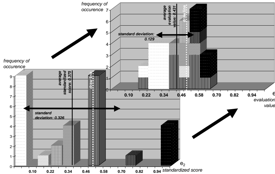
Figure 4.5: Comparison between the score-based evaluation function e_2 and the newly introduced evaluation function e
