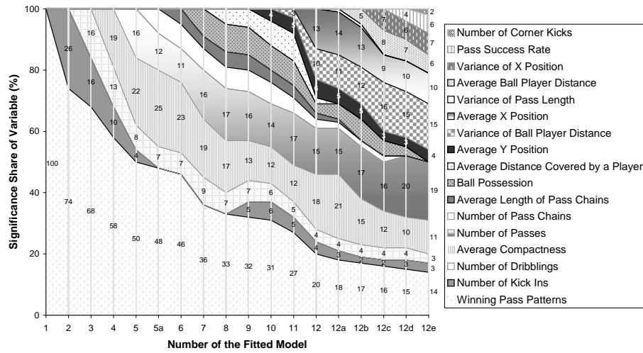
Figure 4.3: Stepwise variable selection with the “Algorithm for Forward Selection Followed by Backward Elimination” using parameters p_E = 0.25 and p_R = 0.30 . In this figure we illustrate the relative importance of variables at successive steps of the algorithm.
