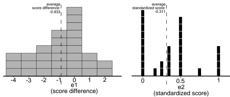
Figure 4.1: Distribution of match evaluation values as calculated by the simple evaluation functions e_1 and e_2
