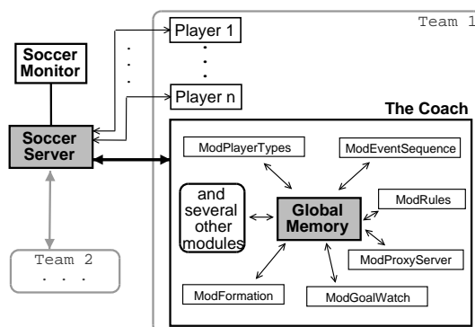
Figure 2.1: The role of the online coach
