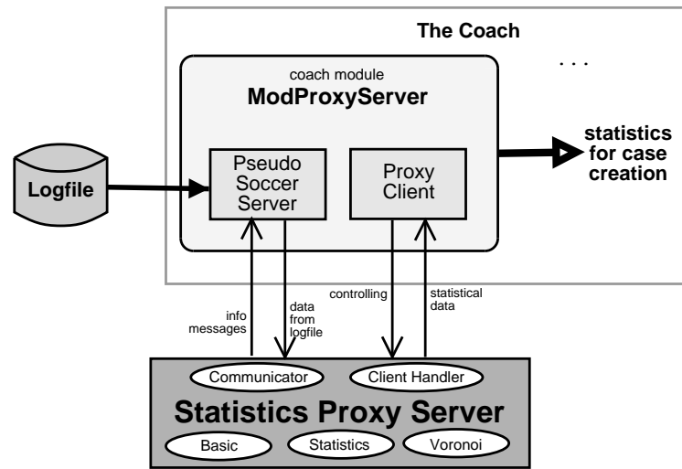
Figure 3.2: Using the Statistics Proxy Server to gain team statistics
