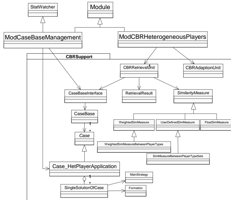
Figure 6.1: Class diagram for the CBR framework
