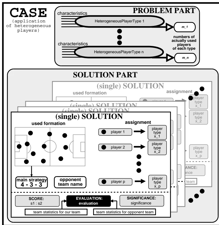
Figure 3.1: The case structure
