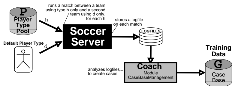
Figure 5.2: Proceeding to generate training data sets
