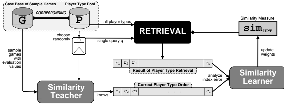
Figure 5.3: Framework for learning the feature weights of sim_{HPT}
