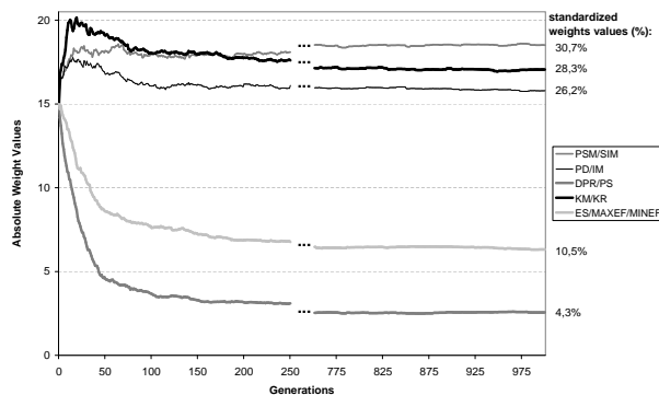
Figure 5.7: Progress of learning – feature weights for the 5 attribute groups
