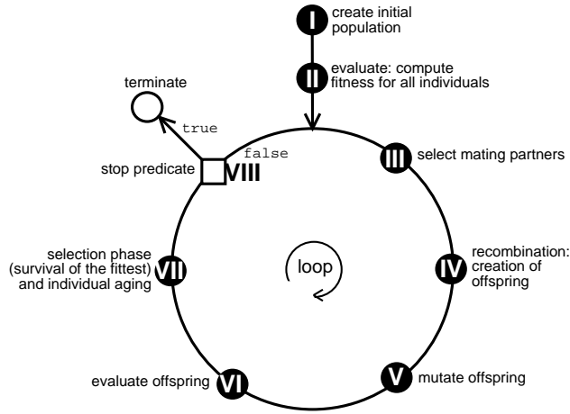
Figure 5.4: Generational loop for a genetic algorithms
