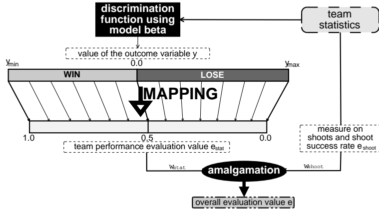
Figure 4.4: Mapping the discriminator's result to a team evaluation assessment
