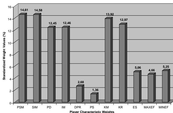
Figure 5.6: Learning result for s = 10 ; the final weights for the 11 player type attributes after 1000 life cycles of the GA weight learner
