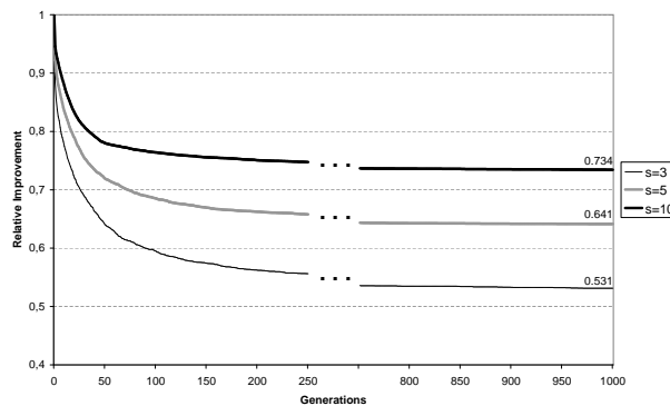
Figure 5.5: Relative improvement of the average index error for different query set sizes
