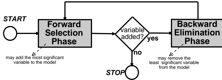
Figure 4.2: Schematic depiction of the “Algorithm for Forward Selection and Backward Elimination”
