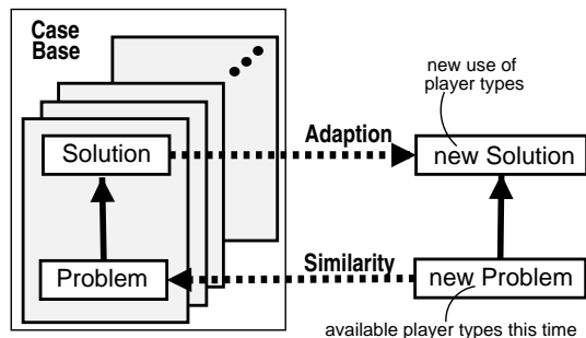
Figure 2.2: Using CBR for the problem of heterogeneous players
